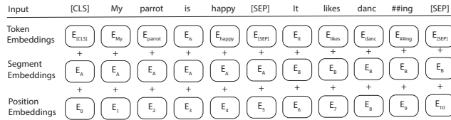
Figure 12.4 Input example for the next sentence prediction pre-training task. [SEP] is a special separator token used to indicate end of sentence. The [CLS] token stands for class , and is used to train the binary classifier, which indicates if sentence B follows sentence A in text or not. The ## marker indicates that the corresponding token is a subword token that should be appended to the token to its left.
