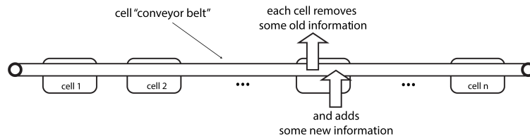
Figure 10.4 Intuition behind the LSTM architecture.
