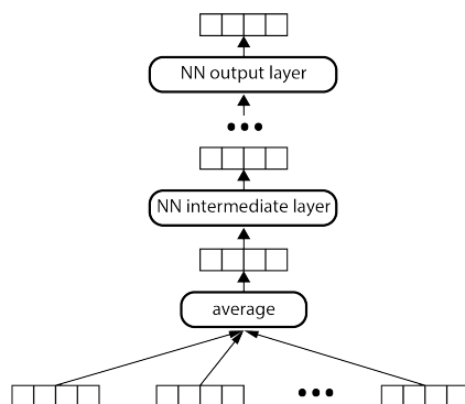
Figure 16.1 Deep averaging network (DAN) for text classification.
