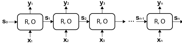
Figure 10.1 “Vanilla” recurrent neural network, where s_i are state vectors, x_i are input vectors, and y_i are output vectors. R and O are functions that compute the next state and the current output vector, respectively.
