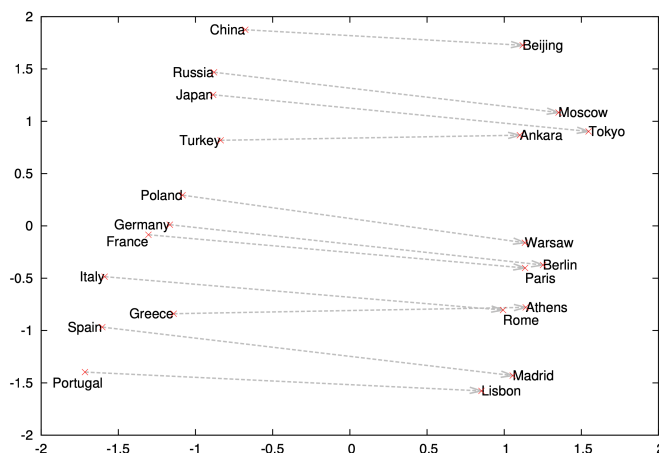
Figure 8.3 Two-dimensional projection of 1000-dimensional vectors learned by word2vec for countries and their capitals (Mikolov et al., 2013b).
