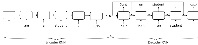
Figure 14.1 An encoder-decoder example for machine translation from English to Romanian, where both encoder and decoder are implemented using RNNs. Two virtual tokens, \text{</s>} and \text{<s>} , indicate end of sentence and beginning of sentence, respectively. The decoder uses the representation generated for the entire input sequence, i.e., the hidden state vector c of the \text{</s>} token in the English sentence, to generate the equivalent Romanian words.
