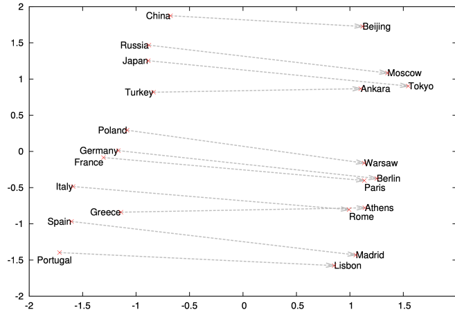
Figure 8.3 Two-dimensional projection of 1000-dimensional vectors learned by word2vec for countries and their capitals (Mikolov et al., 2013a).
