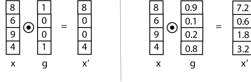
Figure 10.5 Example of a binary gate (left) and gate with real-valued elements (right).
